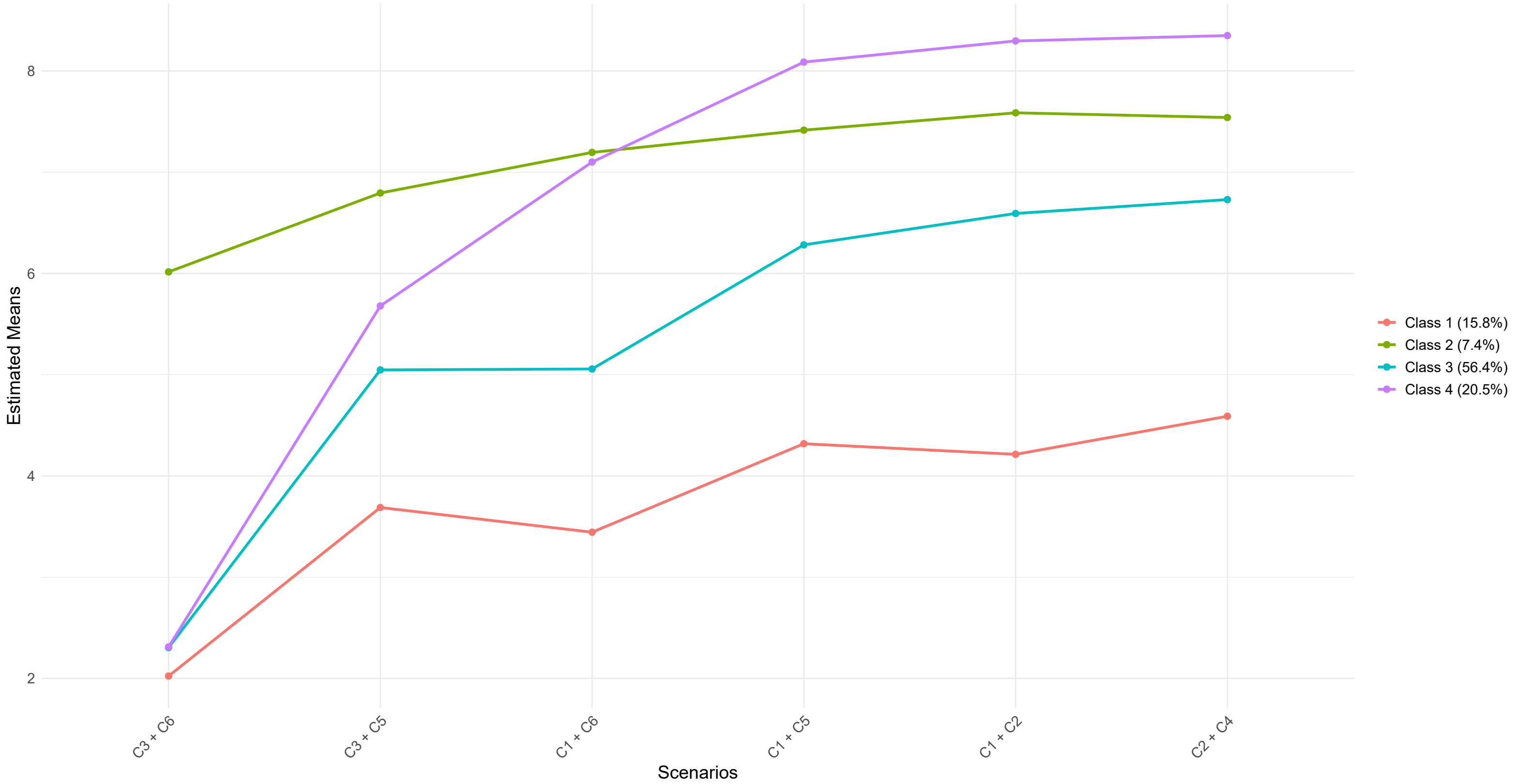
Latent Profiles
